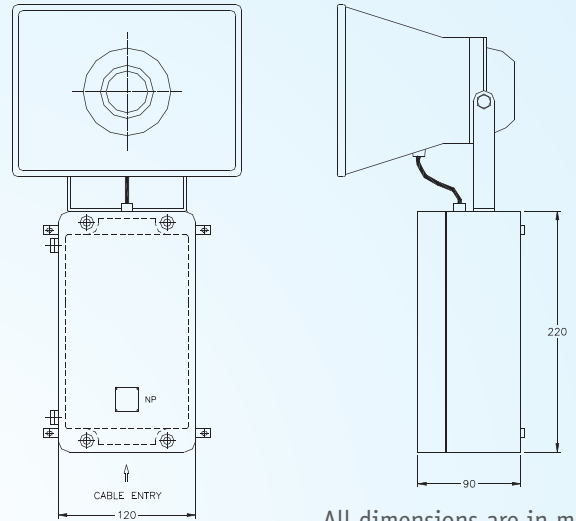
GA Drawing
